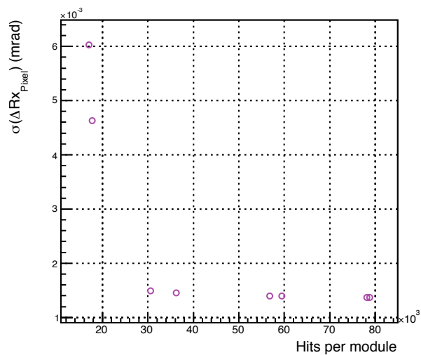
Local Pixel align correction error - \sigma(\Delta Rx) Vs Hits per Module
