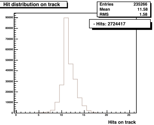
SCT Hit distribution on track
