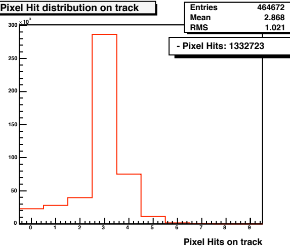
Pixel Hit distribution on track
