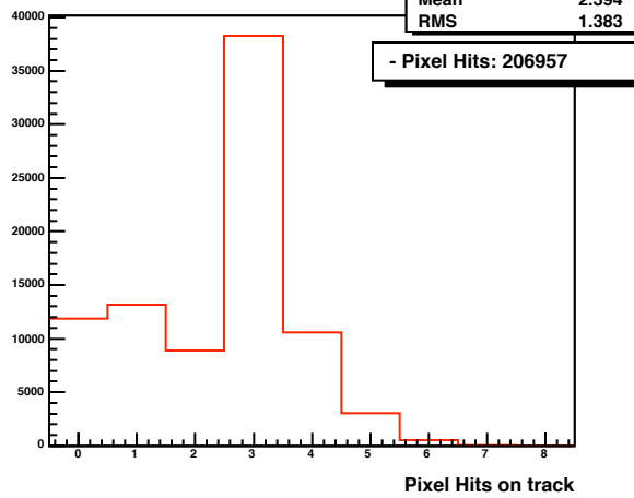
Pixel Hit distribution on track
