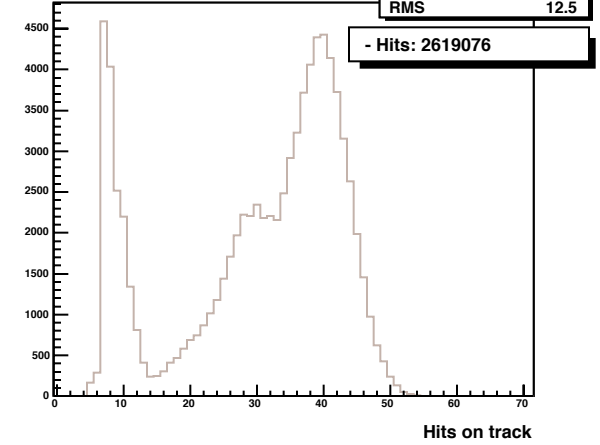
SCT Hit distribution on track
