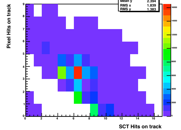
SCT Hit distribution on track
