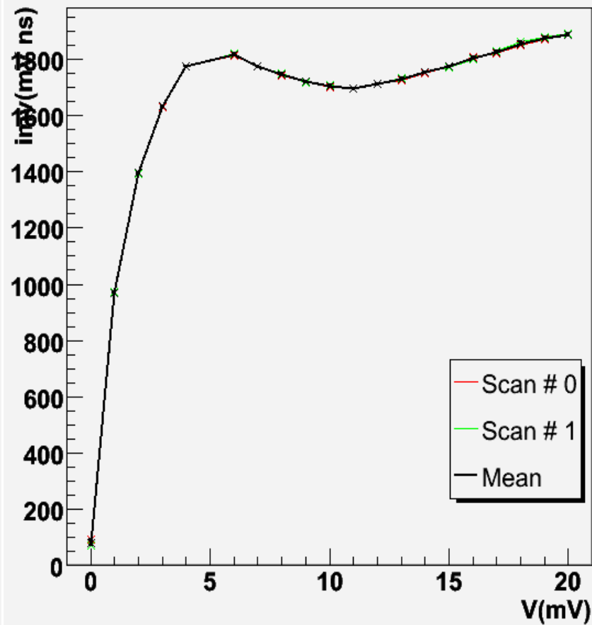
Integral Maximum Value vs Voltage
